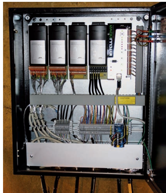
SPM's Intellinova continuous monitoring system delivers easily understood condition information straight to the control room
